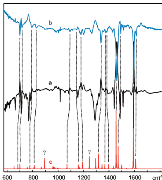
Figure 6. (a) IR spectrum produced by bleaching of o -biphenyl azide in Ar/HCl at 254 nm (negative peaks) and formation of the nitrenium cation 11 (positive peaks); (b) bleaching of 11 (negative peaks) by irradiation at \lambda > 590\text{ nm} ; (c) IR spectrum of 11 calculated by B3LYP/6-31G*.
